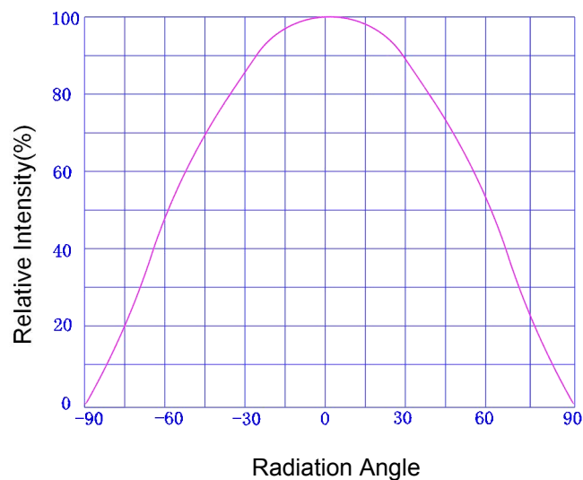
Fig.7- Directivity
